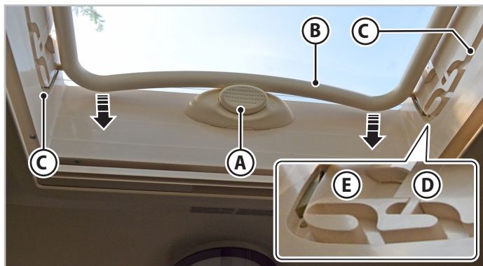
Fig. 6.10 - Vippbar takluke - Type A
